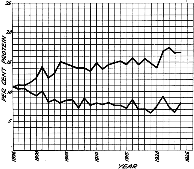
FIGURE 1.—Progress of high-protein and low-protein corn breeding
