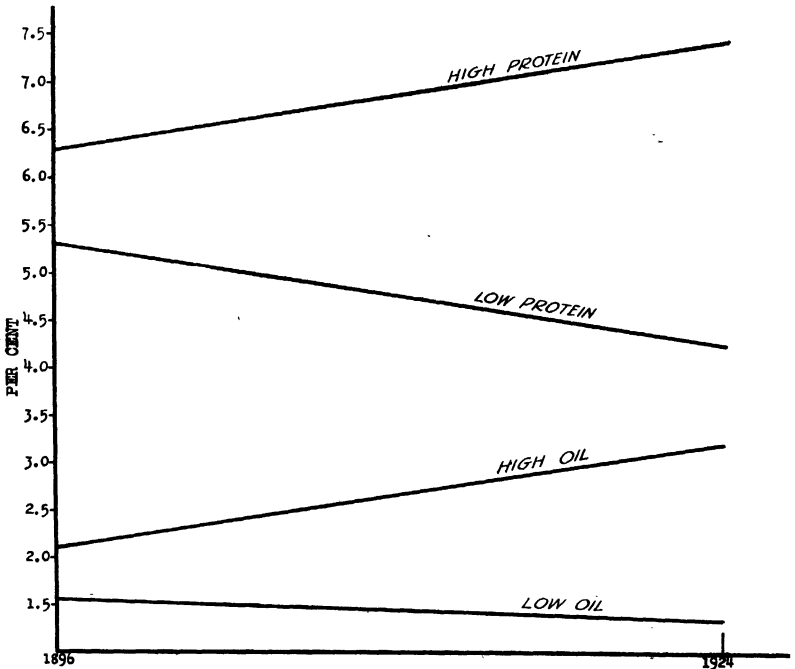
FIGURE 15.—Comparison of the ranges between the highest variate and the lowest variate for high-protein, low-protein, high-oil, and low-oil Illinois corn as expressed by the best fitting straight lines
