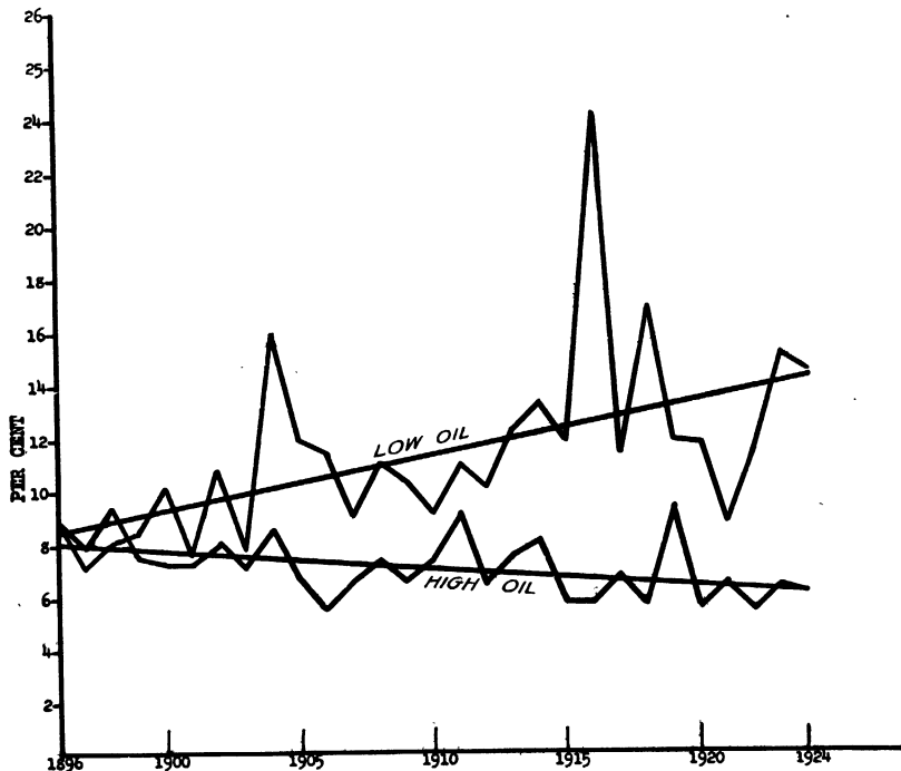
FIGURE 4.—Yearly variations in the oil content of corn and their straight-line trends as measured by the coefficient of variation
