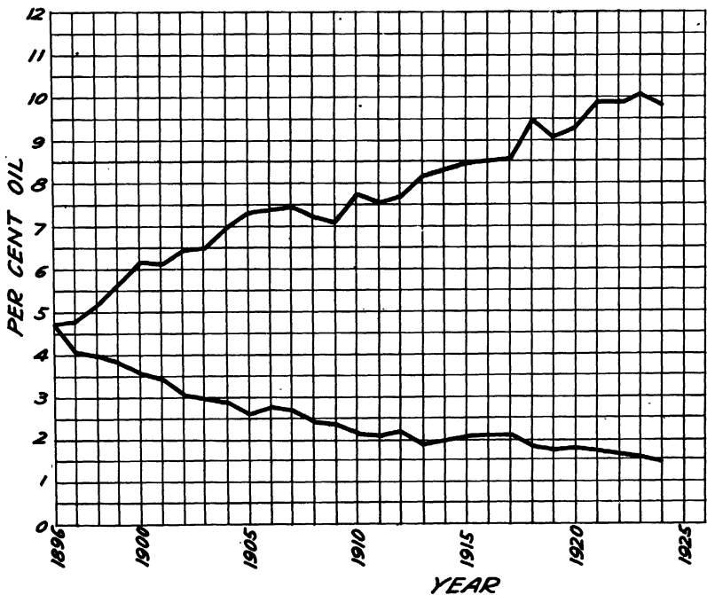
FIGURE 2.—Progress of high-oil and low-oil corn breeding
