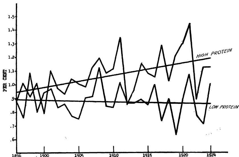
FIGURE 7.—Yearly variations in protein content of corn and their straight-line trends as measured by Weinberg's formula, 1896-1924
