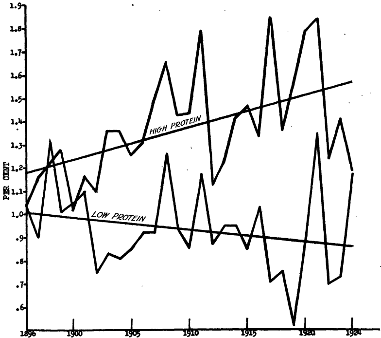
FIGURE 5.—Yearly variations in protein content of corn and their straight-line trends as measured by the standard deviation, 1896-1924
