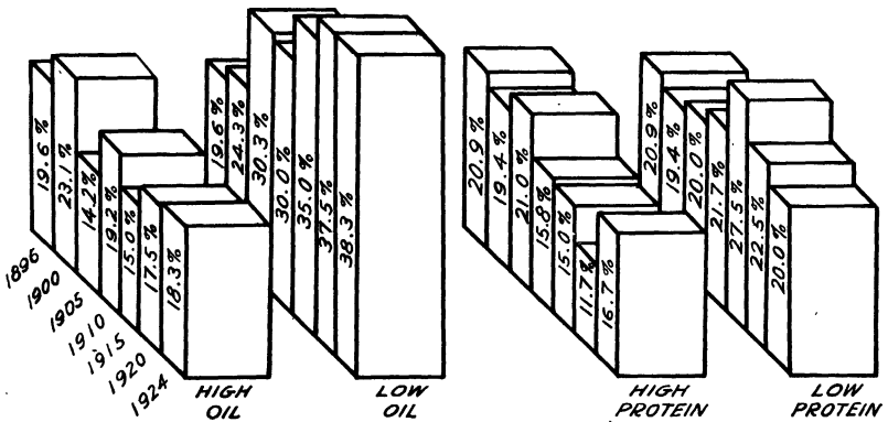
FIGURE 9.—Graphic presentation of the modal classes with respect to the percentage composition of Illinois high and low oil, and high and low protein corn, at periodic intervals between 1896 and 1924
