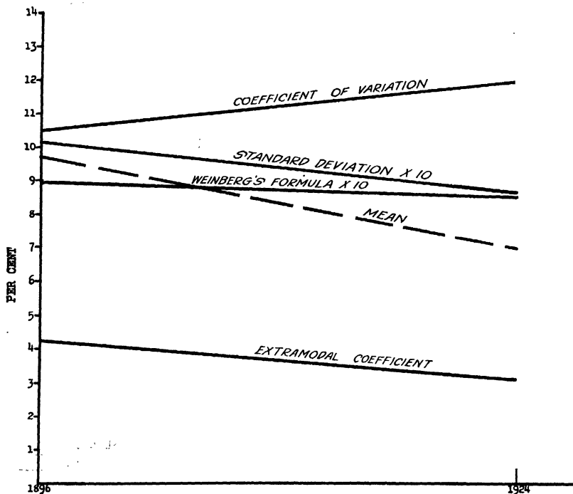
FIGURE 11.—Comparison of four different measures of variation for protein content of Illinois low-protein corn as expressed by the best fitting straight lines: the broken line shows the trend of the mean protein content
