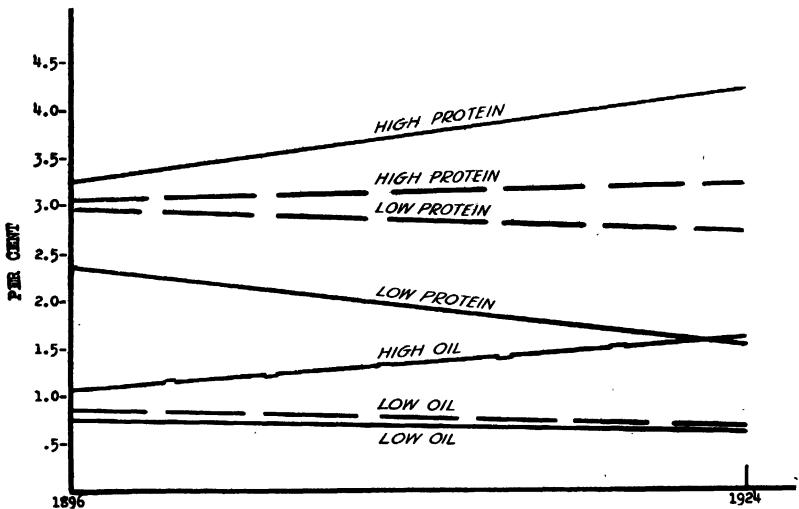
FIGURE 14.—Comparison of the range between the lowest variate and the mean (solid line), and the highest variate and the mean (broken line), for high-protein, low-protein, high-oil, and low-oil Illinois corn as expressed by the best fitting straight lines
