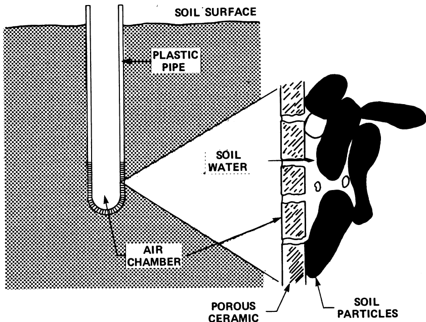
Figure 3.—Cutaway view of a cup-type porous ceramic sampler.
