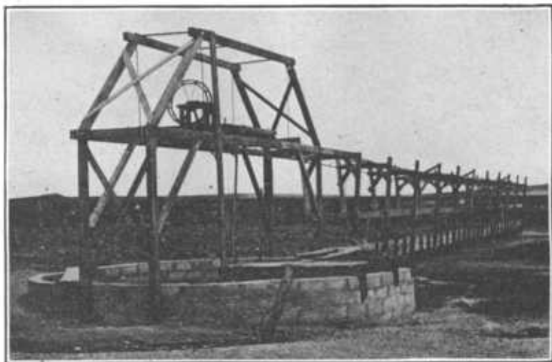
FIG. 6.—A large pit silo with the hoisting and feeding equipment used in connection. The hand hoist is patented. The silage is carried along on the track over the feed troughs. Framework over the troughs is made for a shed. Feeding can be done easily and rapidly with this equipment.
