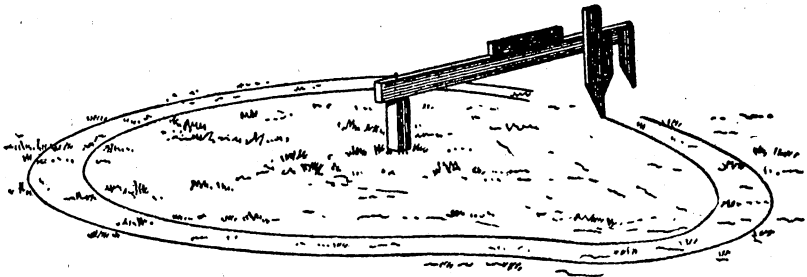
FIG. 1.—Marking off the trench for the curb. Where the ground on which the silo is to be located is not level, the markers can be lengthened by holding a longer board against either marker, as indicated in the figure, moving it up or down to keep it touching the ground, but care must be taken that the scantling is held level.
