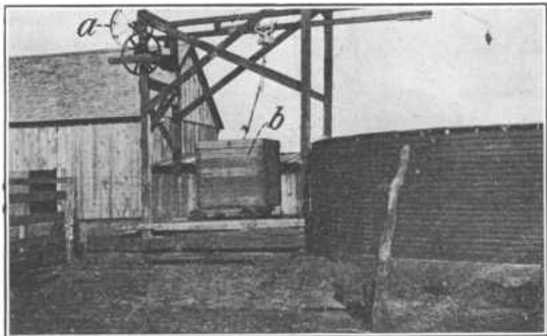
FIG. 4.—A well-enclosed pit silo, showing a combination hand hoist and hay carrier used to lift the silage. An endless rope or chain runs on the wheel "A" by which the windlass is operated. The silage box "B" is transferred to the truck and carried out along the continuous feed trough.
