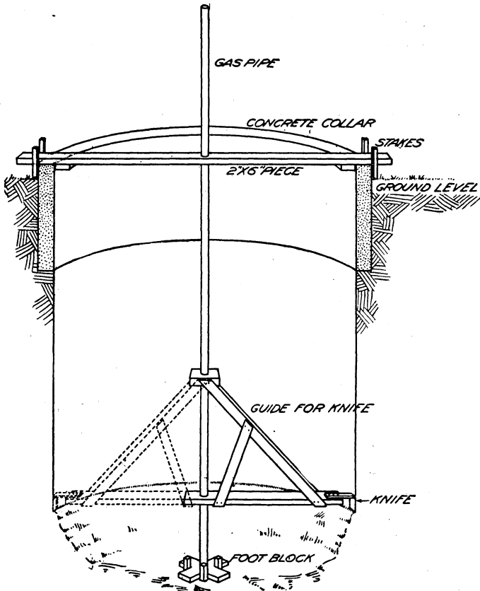
FIG. 2.—Vertical section of a partially constructed pit silo, showing a device for making the wall perpendicular and smooth. (Adapted from Circular No. 6 of the Extension Service of the University of Arizona College of Agriculture.
