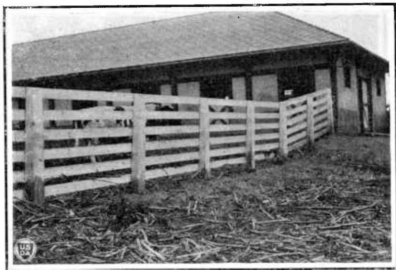
FIG. 3.—Fence of 2 by 6 inch planks on heavy posts.
