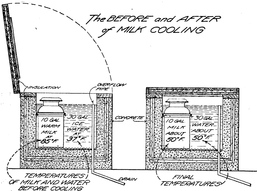
FIG. 3.—Cross section of insulated concrete tank, showing cooling effect of water at a lower temperature.
