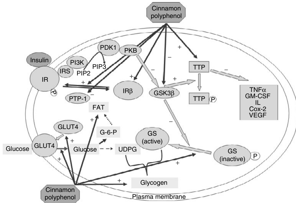
Fig. 3. A model of actions of cinnamon polyphenols (CP) in the insulin signal transduction pathway leading to beneficial effects in subjects with glucose intolerance or type 2 diabetes: (1) CP activate insulin receptors (IR) by increasing their tyrosine phosphorylation activity and by decreasing phosphatase activity that inactivates the receptor; (2) CP increase the amount of insulin receptor- \beta and GLUT4 proteins; (3) CP increase glycogen synthase activity and glycogen accumulation; (4) CP decrease glycogen synthetase (GS) kinase-3 \beta (GSK3 \beta ) activity; (5) CP increase the amount of tristetraprolin (TTP) protein; (6) CP may increase the activity of TTP by decreasing its phosphorylation through inhibition of GSK3 \beta activity. IRS, insulin receptor substrate; PI3K, 1-phosphatidylinositol 3-kinase; PIP2, phosphatidylinositol 4,5-bisphosphate; PIP3, phosphatidylinositol 3,4,5-trisphosphate; PTP-1, protein tyrosine phosphatase-1; PDK1, phosphatidylinositol-dependent protein kinase 1; FAT, fat; G-6-P, glucose 6-phosphate; PKB, protein kinase B; UDPG, uridine diphosphoglucose; GM-CSF, granulocyte-macrophage colony-stimulating factor; Cox2, cyclooxygenase-2; VEGF, vascular endothelial growth factor; -, negative effect; +, positive effect. (From Cao et al. (43) .)
